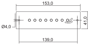
8 LED Strip
