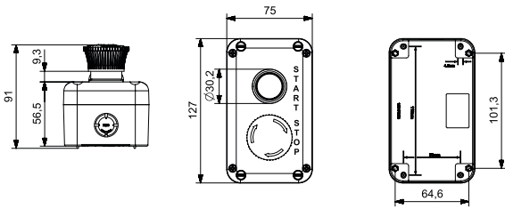
Flush Head Actuator/Mushroom Head Actuator Push Turn Type
