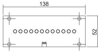
12 LED Strip
